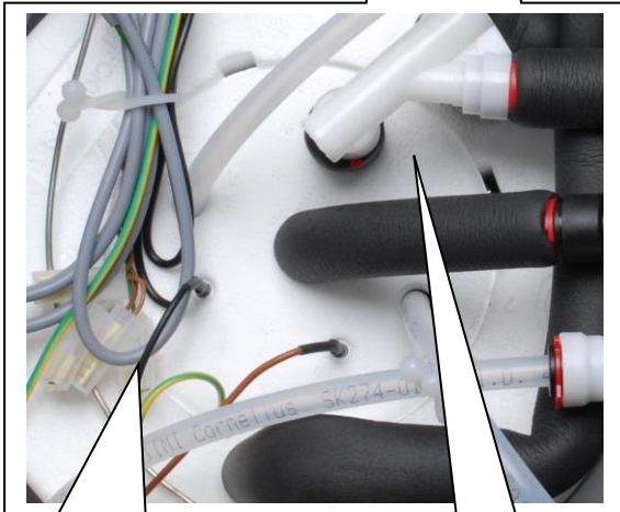
Level probe for pump control min = brown max=black
