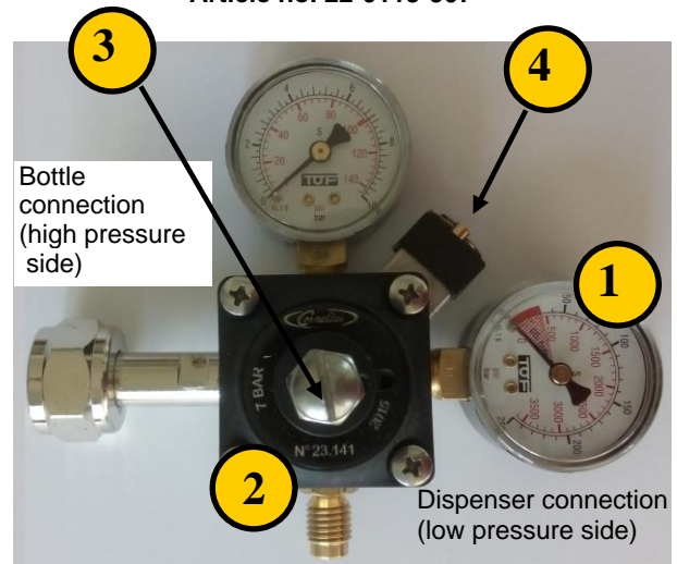
CO 2 regulator Article no. 22-0113-507
